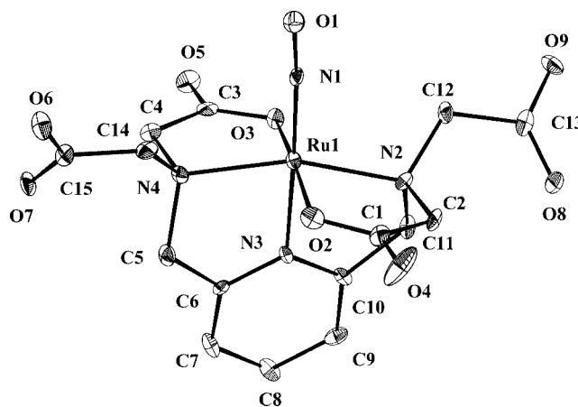
Figure 1. An ORTEP view of the structure of 38 , showing the atom-labelling scheme and 50% thermal ellipsoids.
